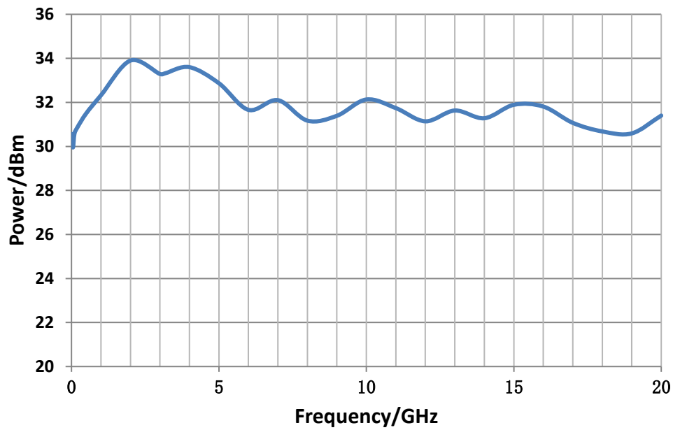
Max. output power (option H06)
