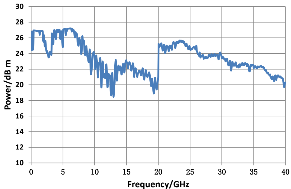
Max. output power (option H05)
