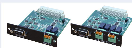
Single and dual channel digital I/O and analog input control cards
