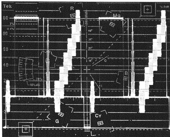
1750A, 2H waveform display.
