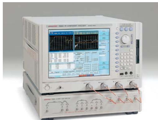
Combination with the R3968 multi-port test set
